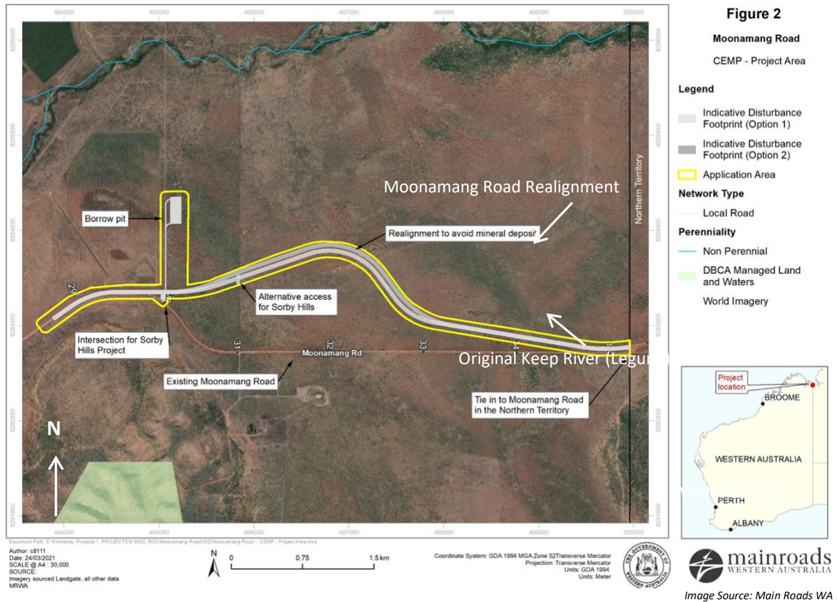
Figure 5 - Moonamang Road Realignment
